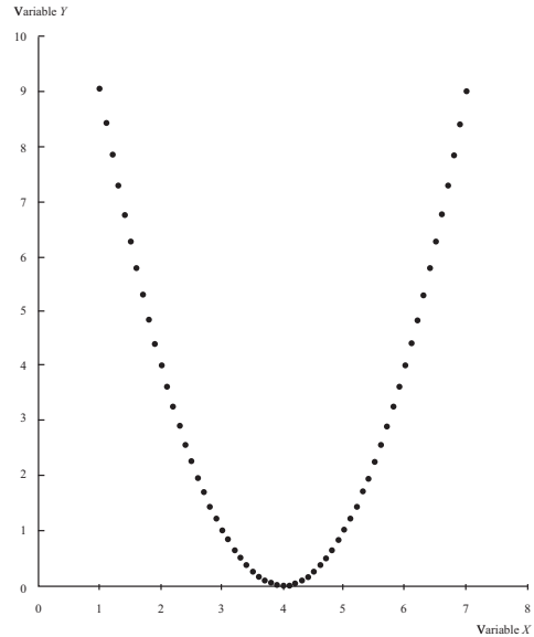
D. Variables with a Strong Nonlinear Association
