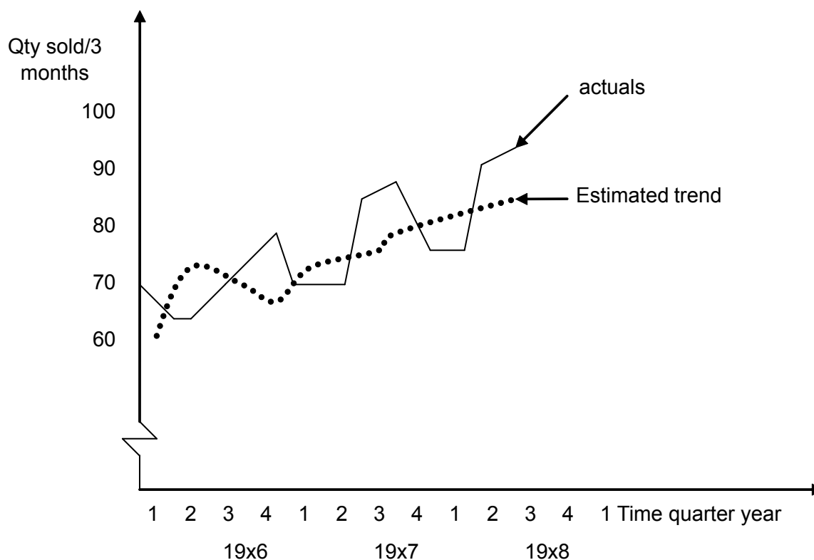
Diagram 5.12 CD Plc actual and deseasonalised sales per 3 months
