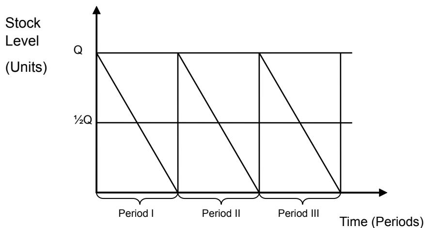
EOQ graph 2
